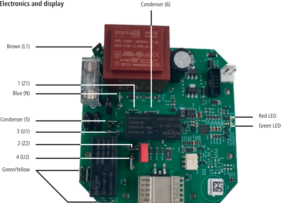
Figure 5: Circuit board connection diagram with capacitor - MaxiSwing
